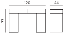
Toilette a terra P=44 H=77
